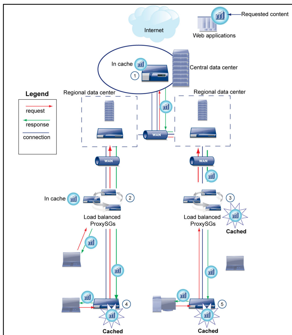
Figure 43–3 How forwarding can leverage object caching to prevent multiple requests to the Internet and over WAN links
