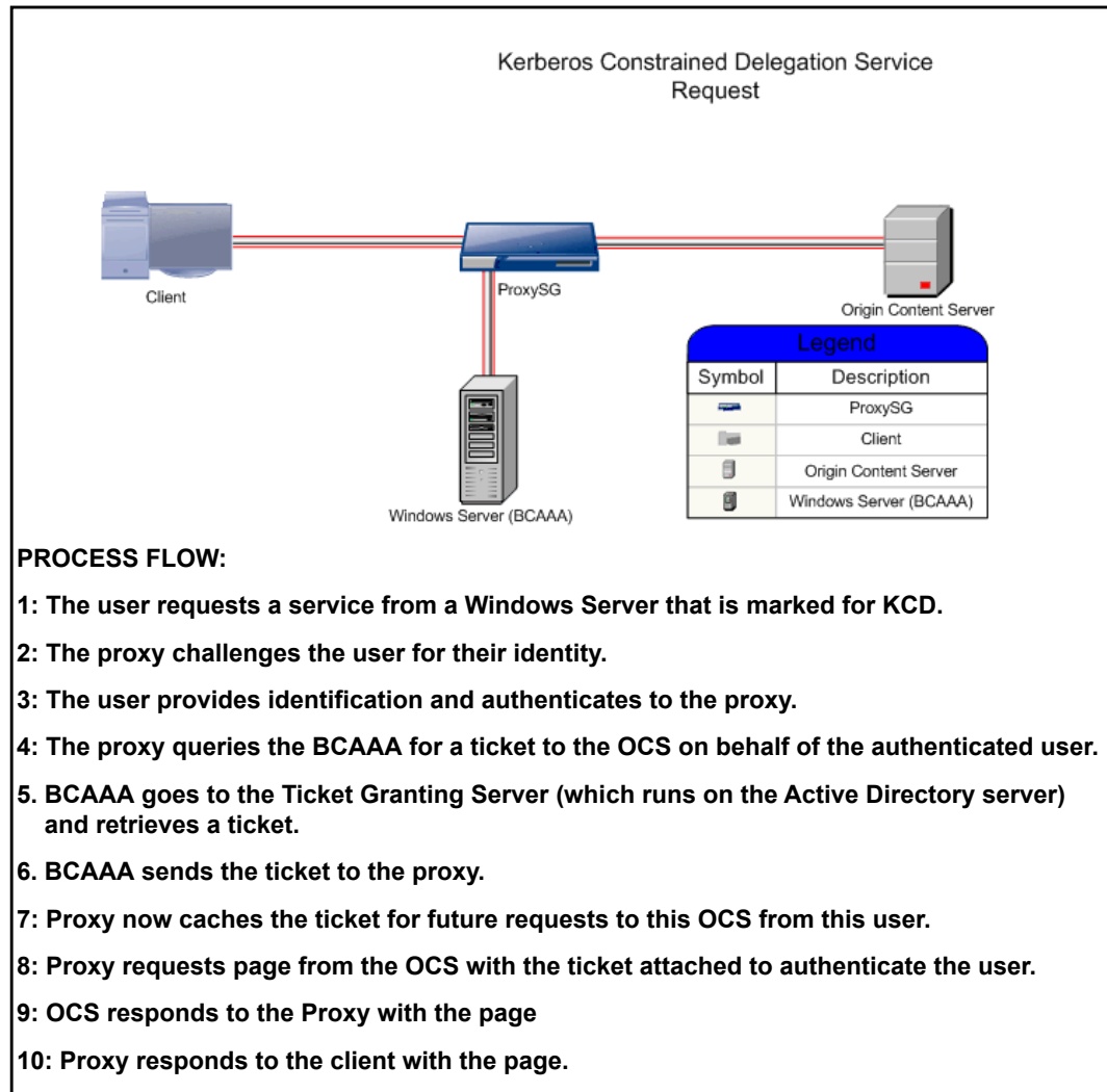
Figure 54–1 Kerberos Constrained Delegation service request process.
