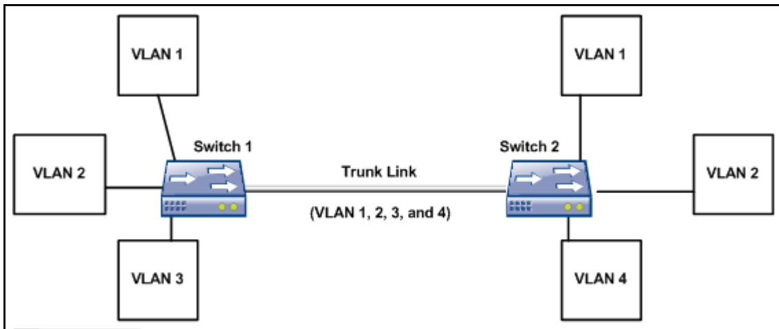
Figure 67–4 Two switches connected by a trunk
