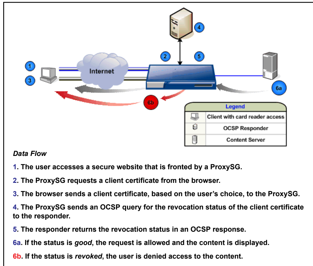
Figure 61–1 Reverse Proxy Scenario
