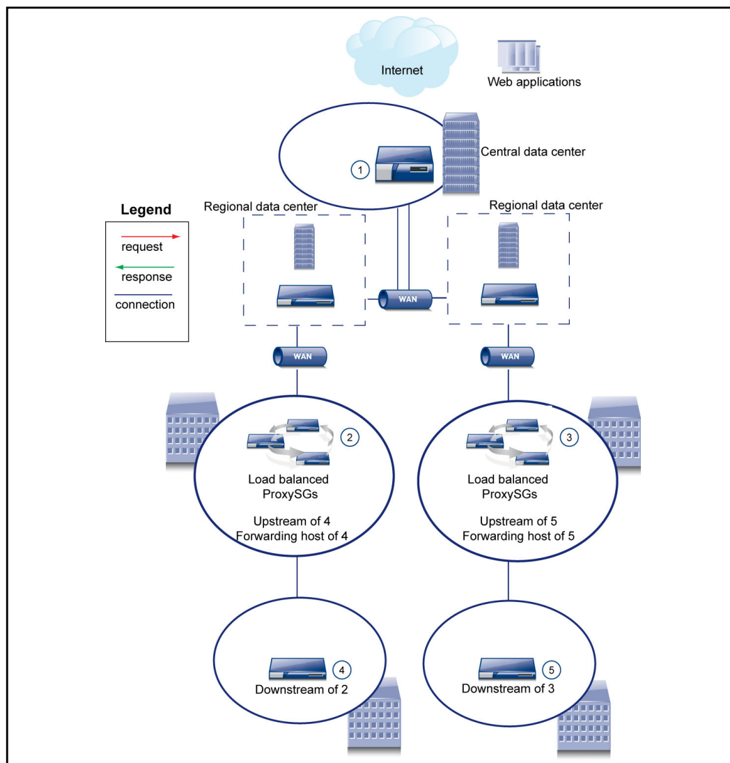
Figure 43-2 Example ADN network that uses forwarding
