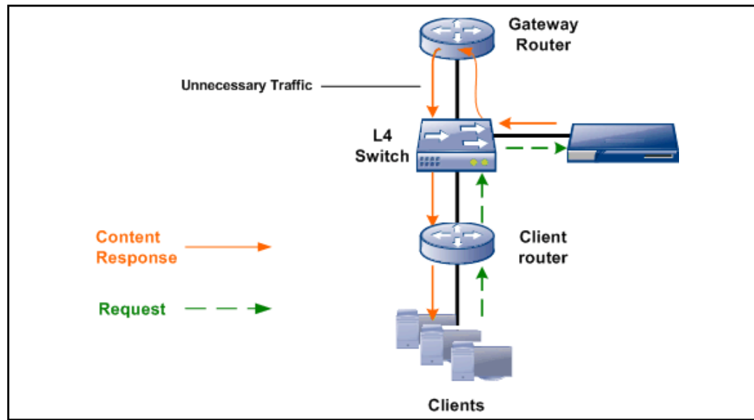
Figure 35–2 Effects of sending client response to the default gateway
