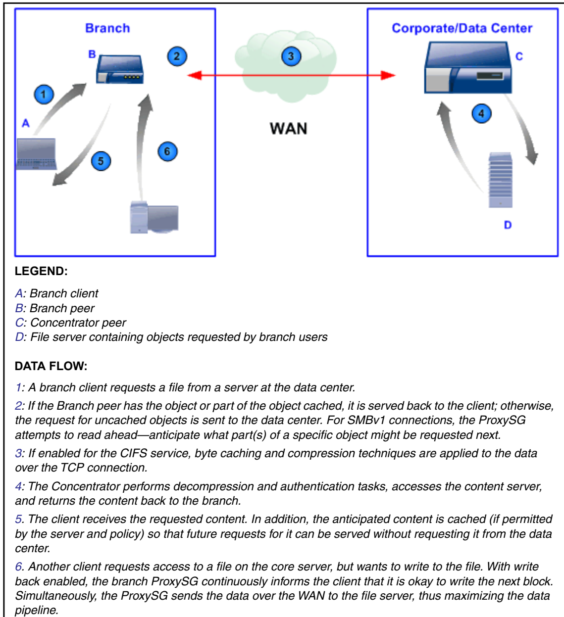
Figure 10–1 CIFS Proxy Traffic and Flow Diagram
