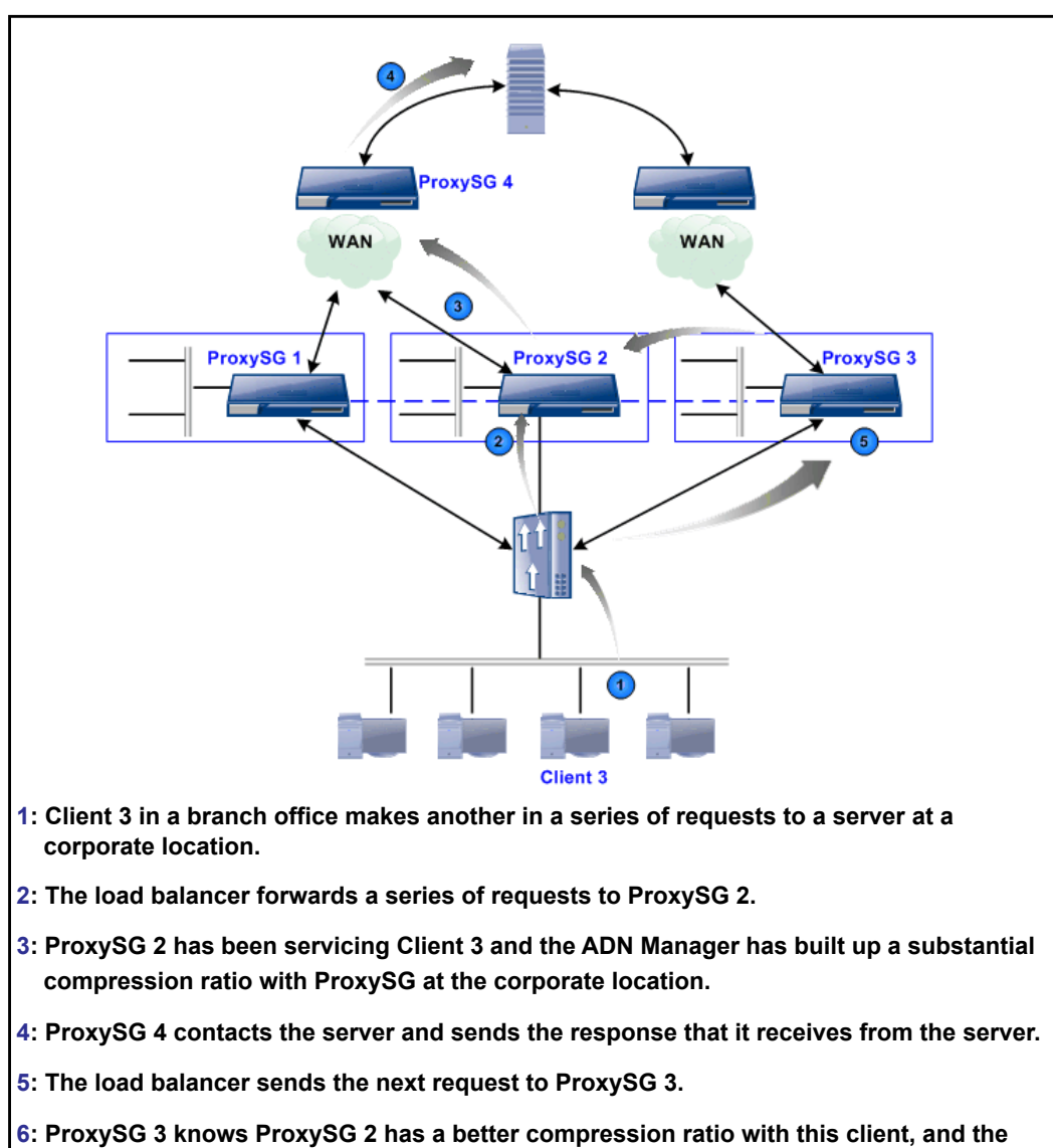
Figure 42–4 ADN Transparent Tunnel load balancing with Connection Forwarding enabled
