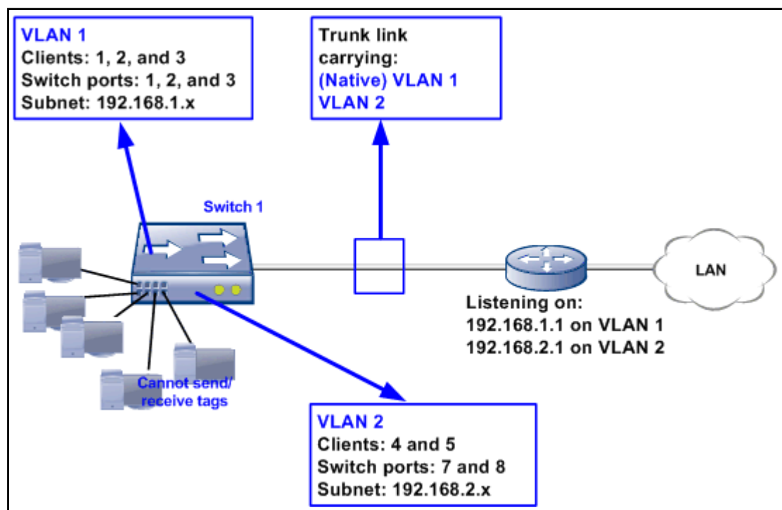
Figure 67–5 A switch broadcasting native and regular VLAN traffic over a trunk
