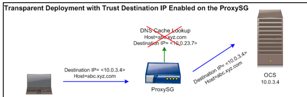
Figure 7–1 No DNS lookup occurs; the transactions goes straight to the OCS.
