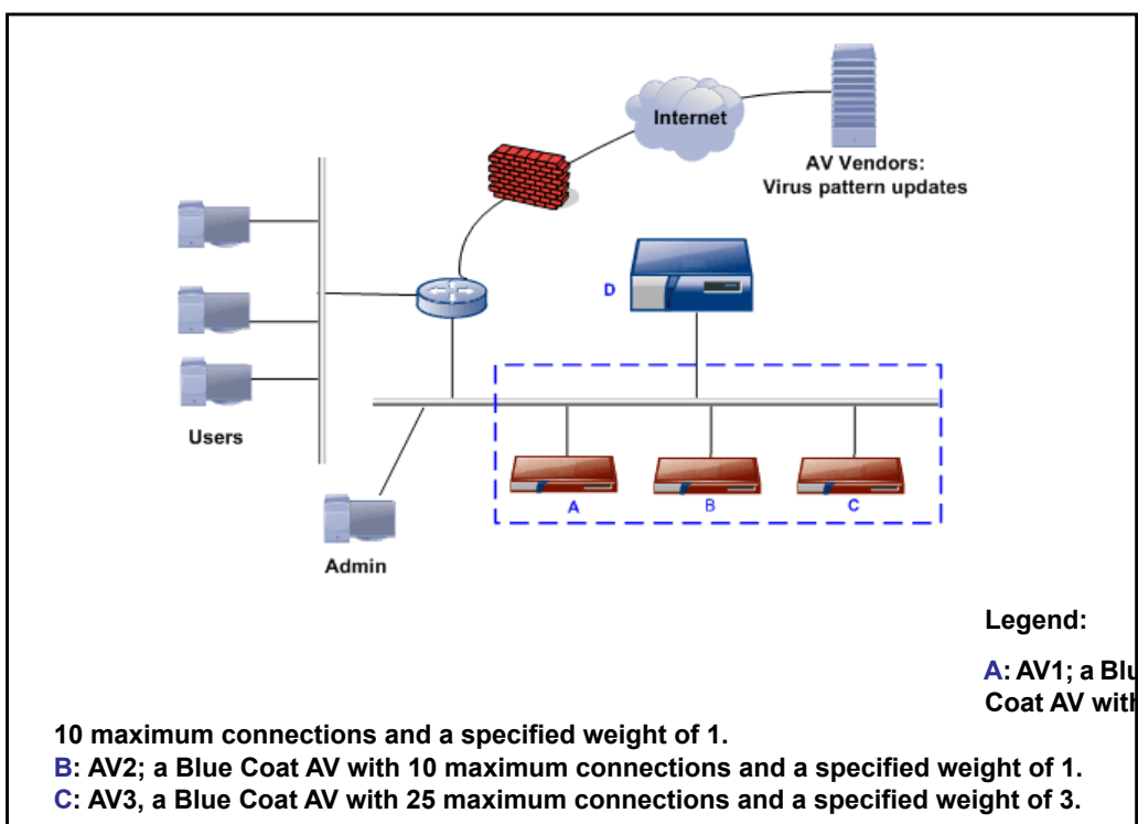
Figure 23–1 ICAP Service Group
