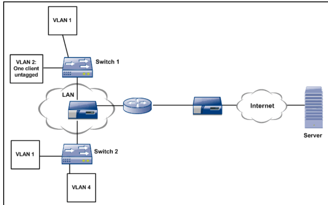
Figure 67-6 ProxySG appliance deployed between two switches
