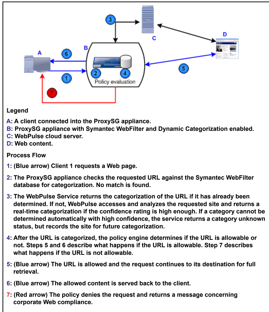
Figure 20–2 WebFilter with Dynamic Categorization Content Enabled (default)
