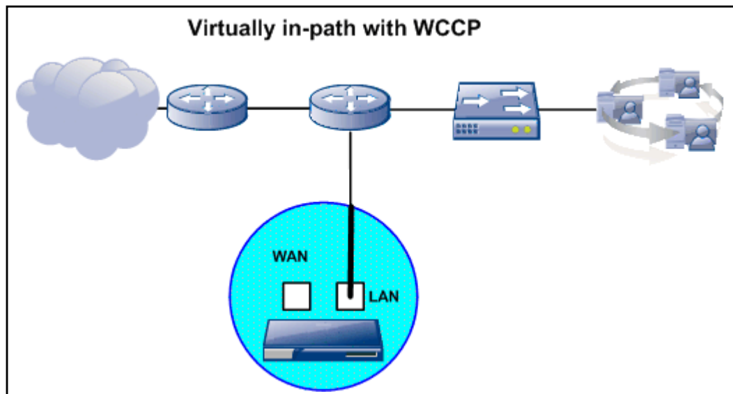
Figure 67–2 Connecting the LAN interface to a router with WCCP.
