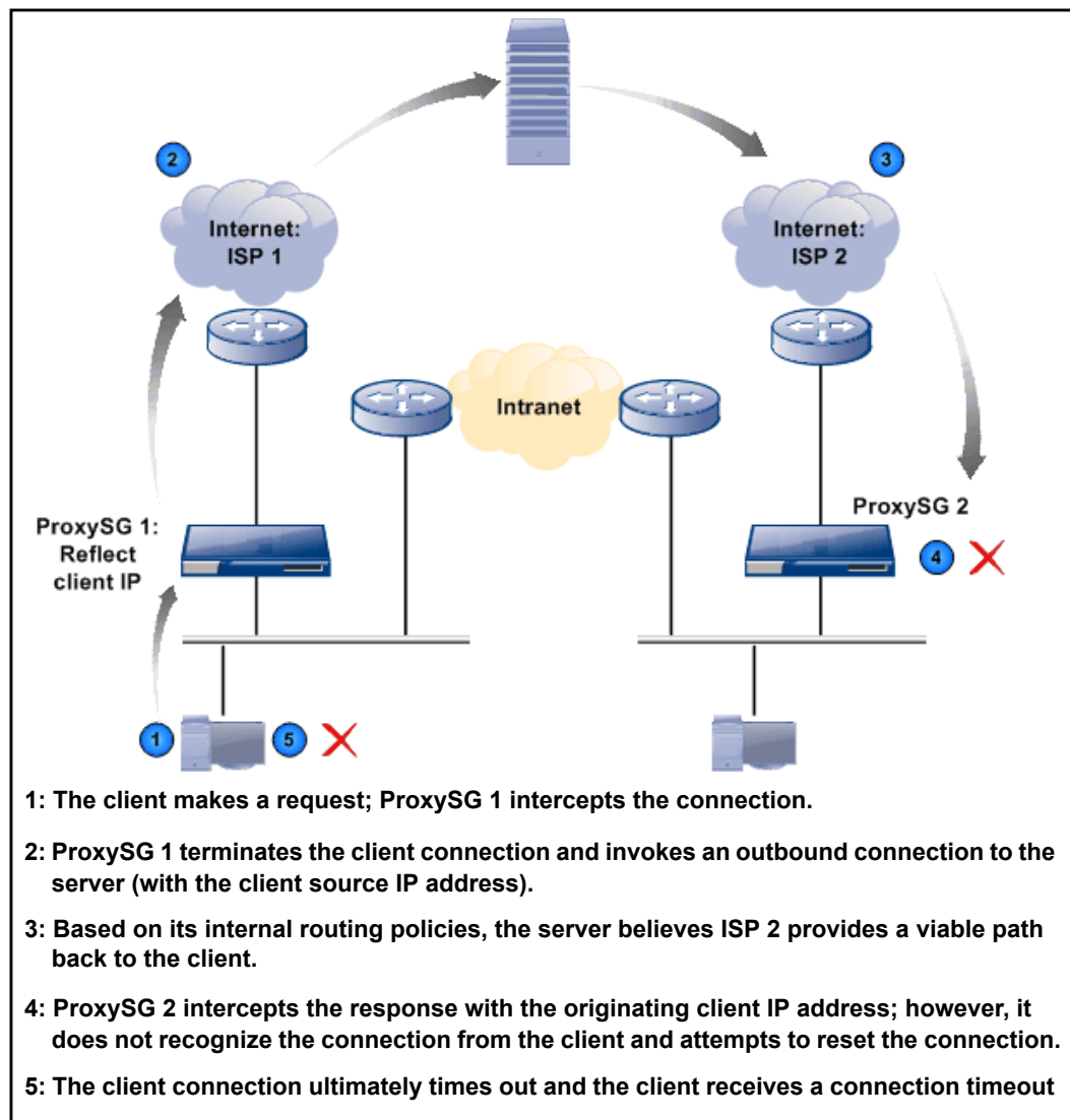
Figure 42–1 Multiple ProxySG appliances in an asymmetric routing environment
