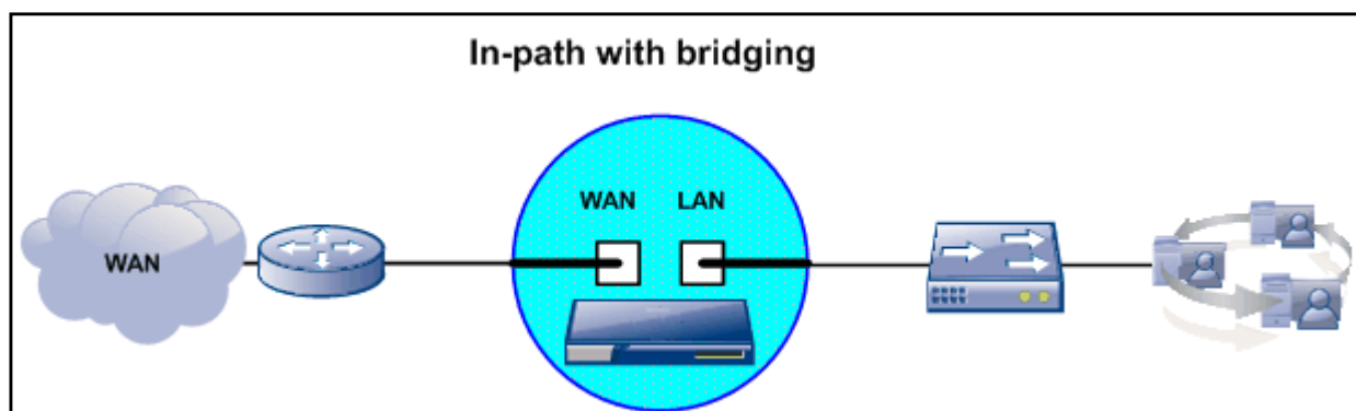
Figure 67–1 Connecting WAN and LAN interfaces in-path with bridging.
