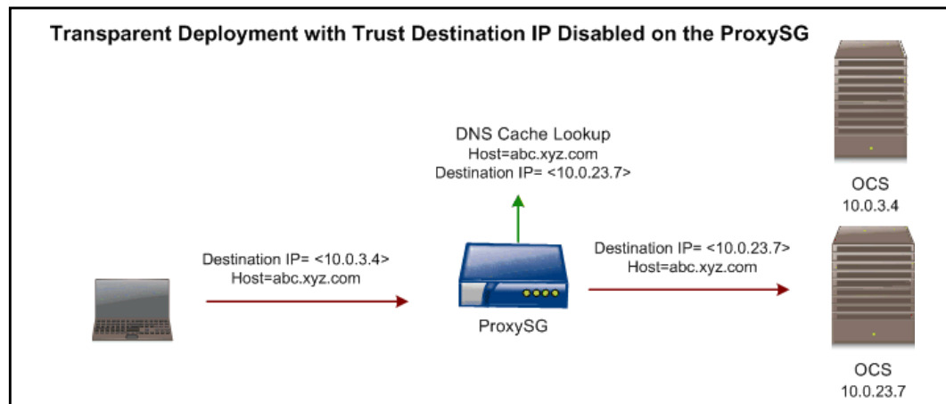
Figure 7–2 The ProxySG initiates a DNS lookup and initiates a new connection to the server. The ProxySG cannot trust the client-provided destination IP address in the following situations:
