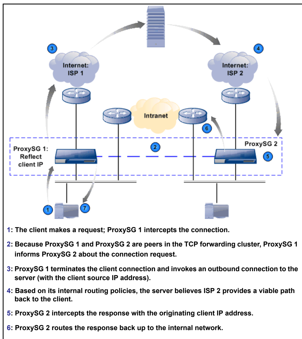
Figure 42–2 ProxySG appliances share TCP connection information
