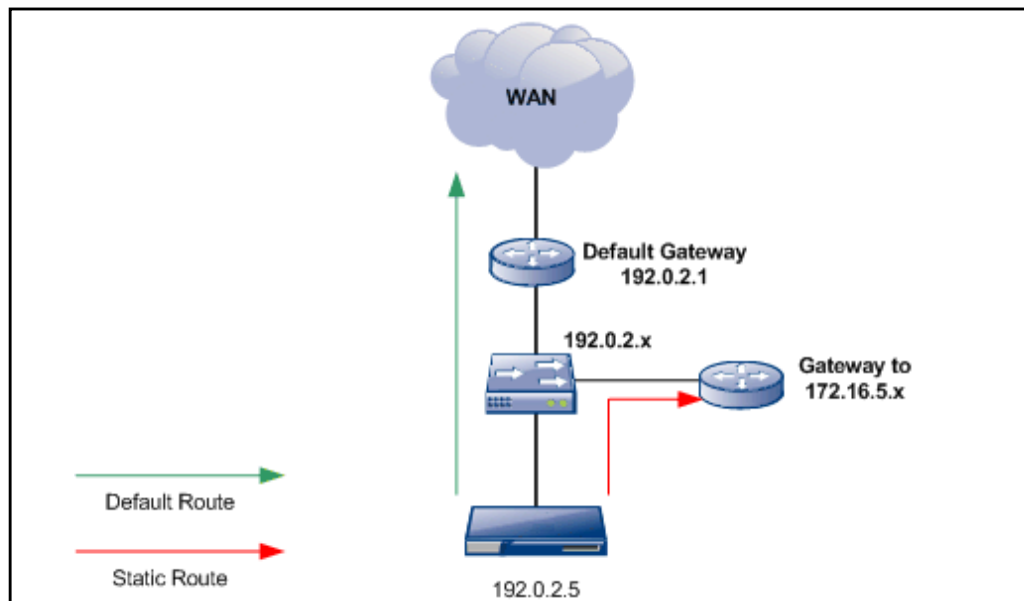
Figure 35–1 Network example of default and static route
