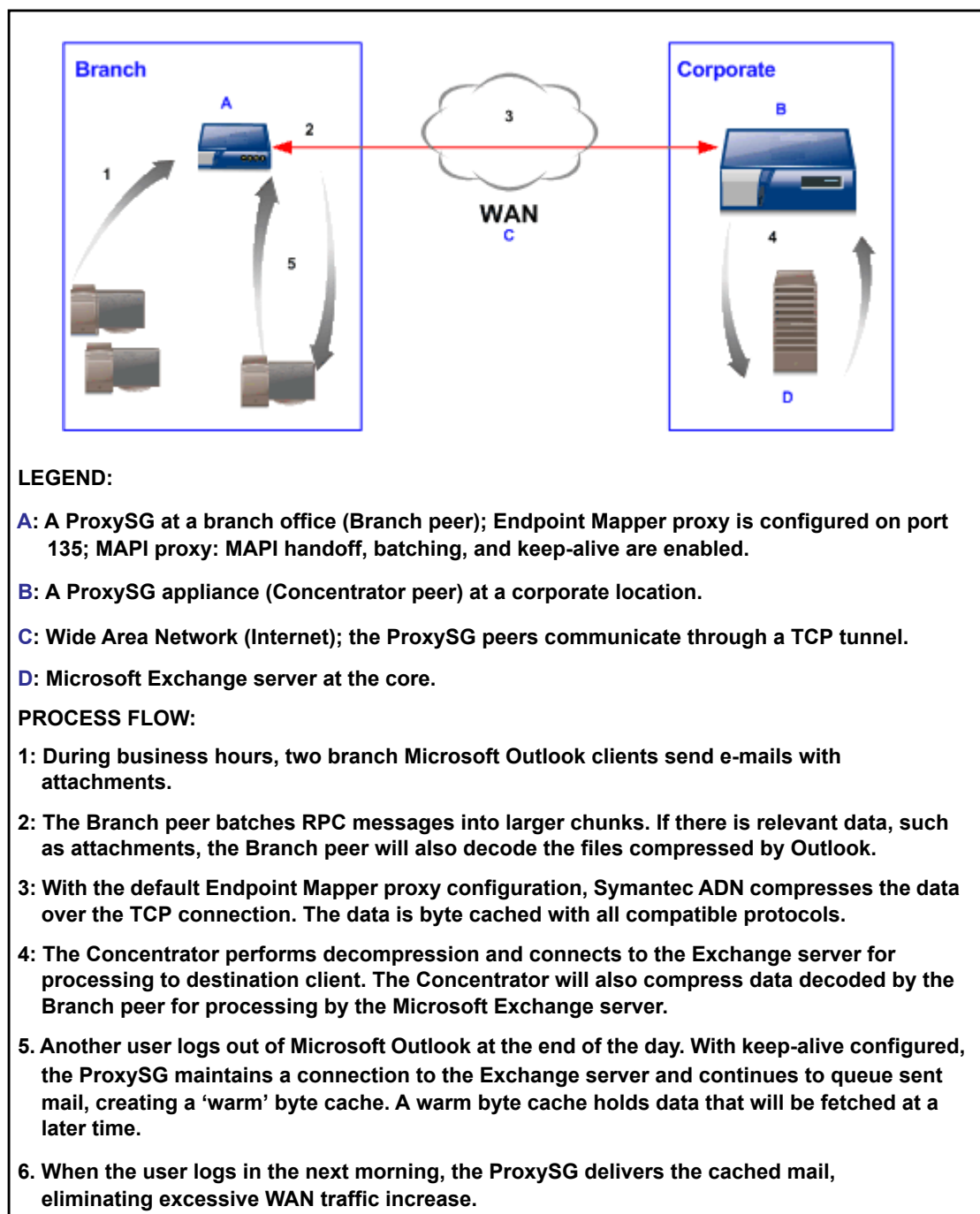
Figure 11–1 MAPI Proxy Deployment and Flow Diagram
